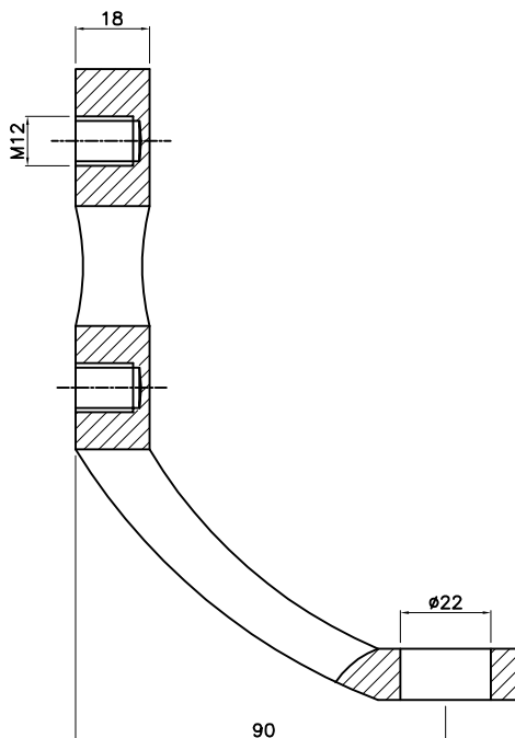
LEFT FITTING
